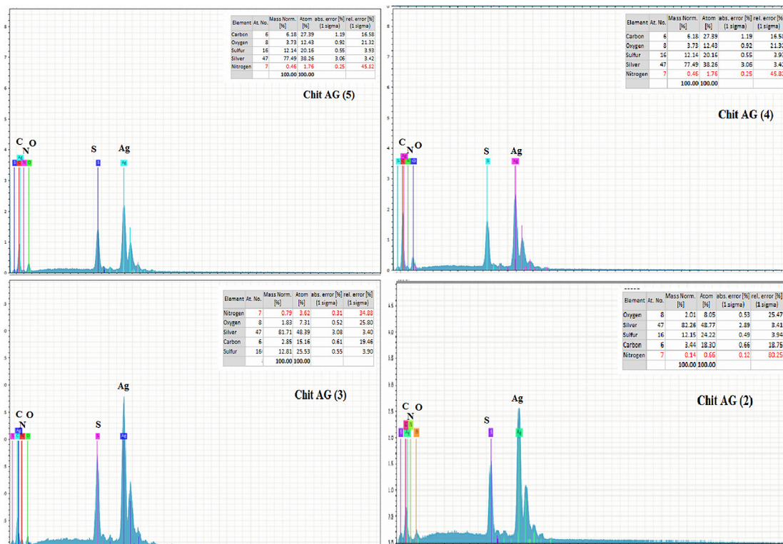
Figure 3a. Representing the EDX of Chit AG (2), Chit AG (3), Chit AG (4), Chit AG (5).
